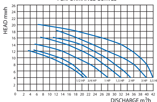
PERFORMANCE CURVES
